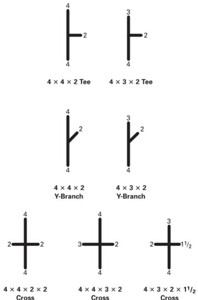
Fig. 1 Identification of Reducing Fittings
